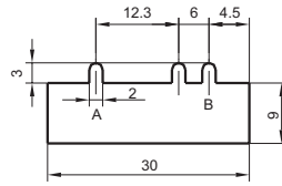
F43( h=1, R=600 ), F44( h=2, R=300 )
